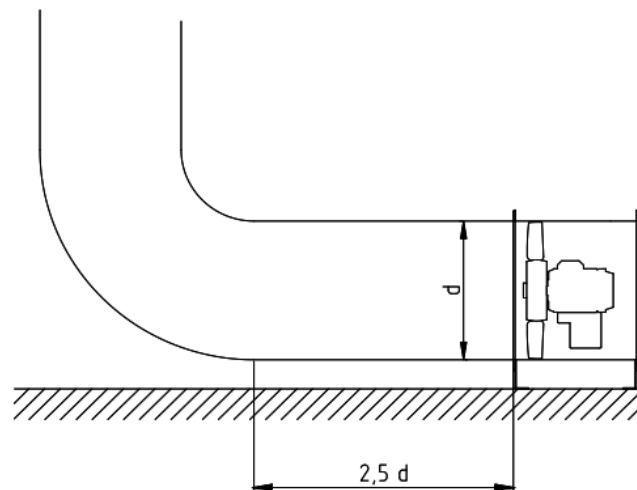
Fig. 5-10 Minimum installation distances with inlet duct
