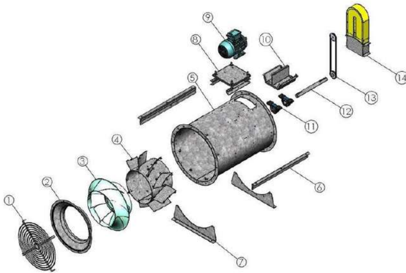
Fig. 2-10 MXC fan components indicated
