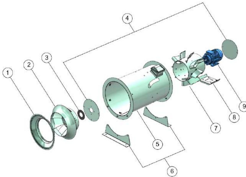
Fig. 2-11 MXC-Bi fan components indicated
