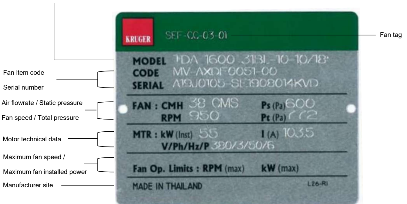
Fig. 2-4 Key to reading fan name plate
