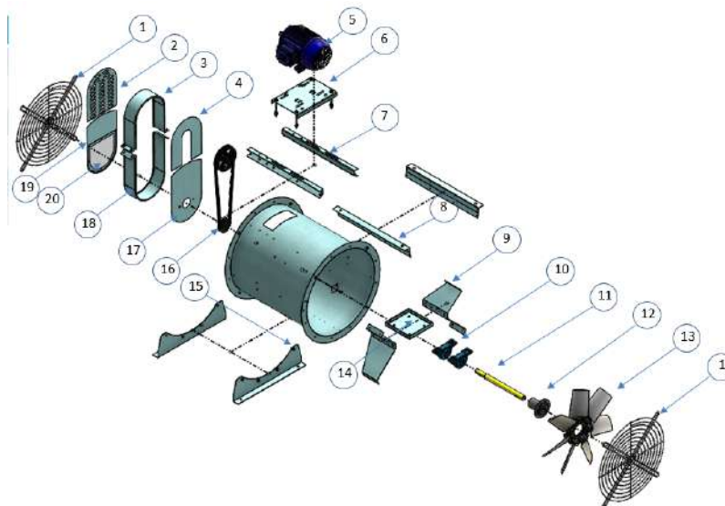
Fig. 2-9 TBE fan components indicated
