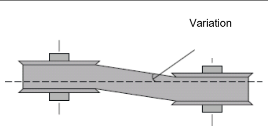
Fig. 9-3 Parallel misalignment
