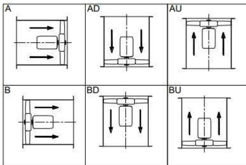
Fig. 2-2 Flow indications
