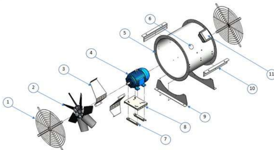
Fig. 2-5 TDA fan components indicated
