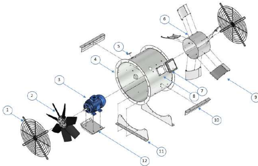
Fig. 10-1 Exploded view of version 4 fan
