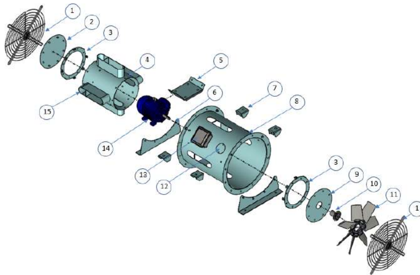
Fig. 2-7 TDB-II fan components indicated
