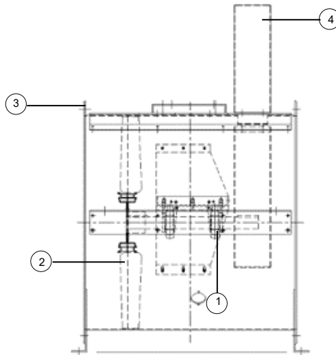
Fig. 5-4 Assembly of version 1 axial fans
