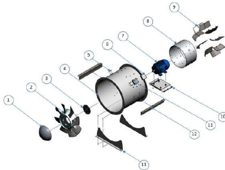
Fig. 2-8 MXA fan components indicated
