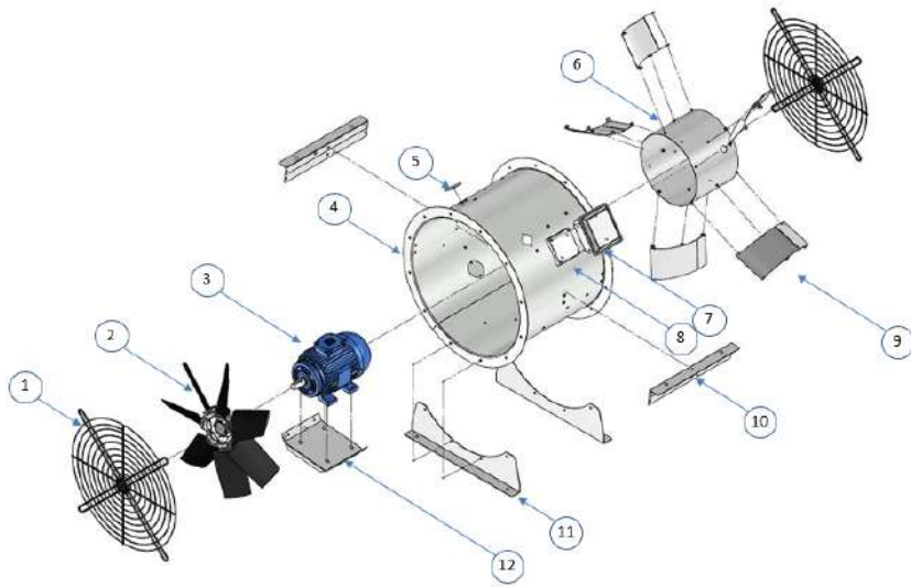
Fig. 2-6 TDA-V fan components indicated
